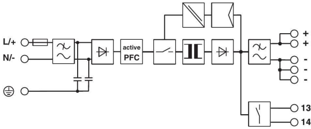
Figure 2 Block diagram
